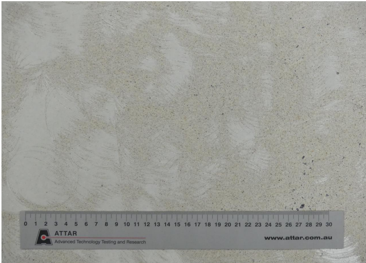
Figure 1: Dulux Avista Extended Wear Sealer with Slip Reducing Additive applied to steel trowel finish concrete
